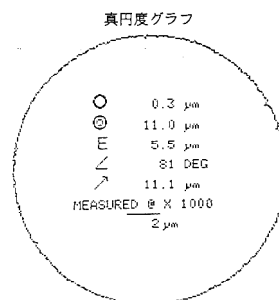
Circularity of the Covered Plunger
