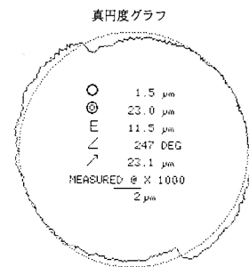
Circularity of the normal plunger
